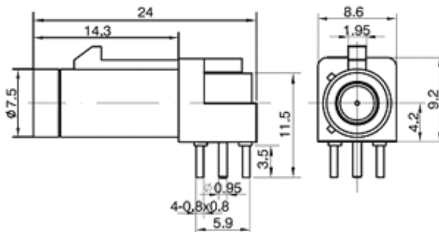
FAKRA SMB-R-M-RA-P-4
